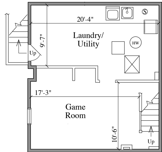
BASEMENT 504 SQ. FT.
