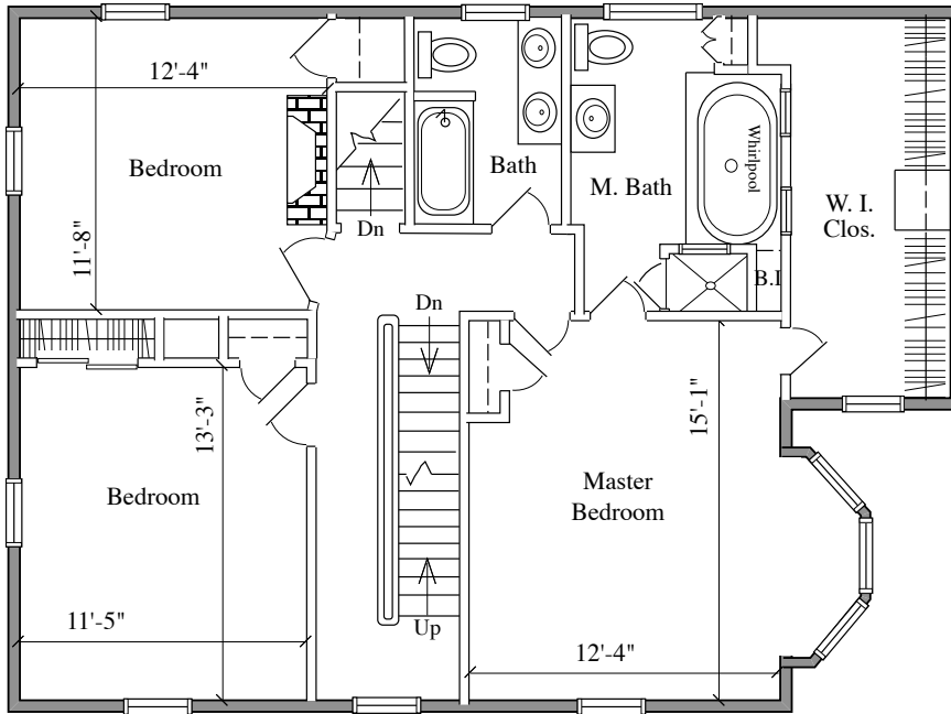
SECOND FLOOR 1,006 SQ. FT.
