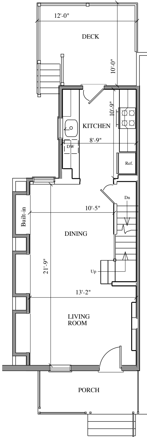
FIRST FLOOR 465 SQ. FT.
