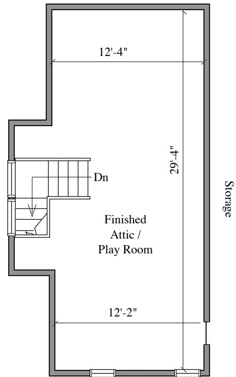
THIRD FLOOR 445 SQ. FT.
