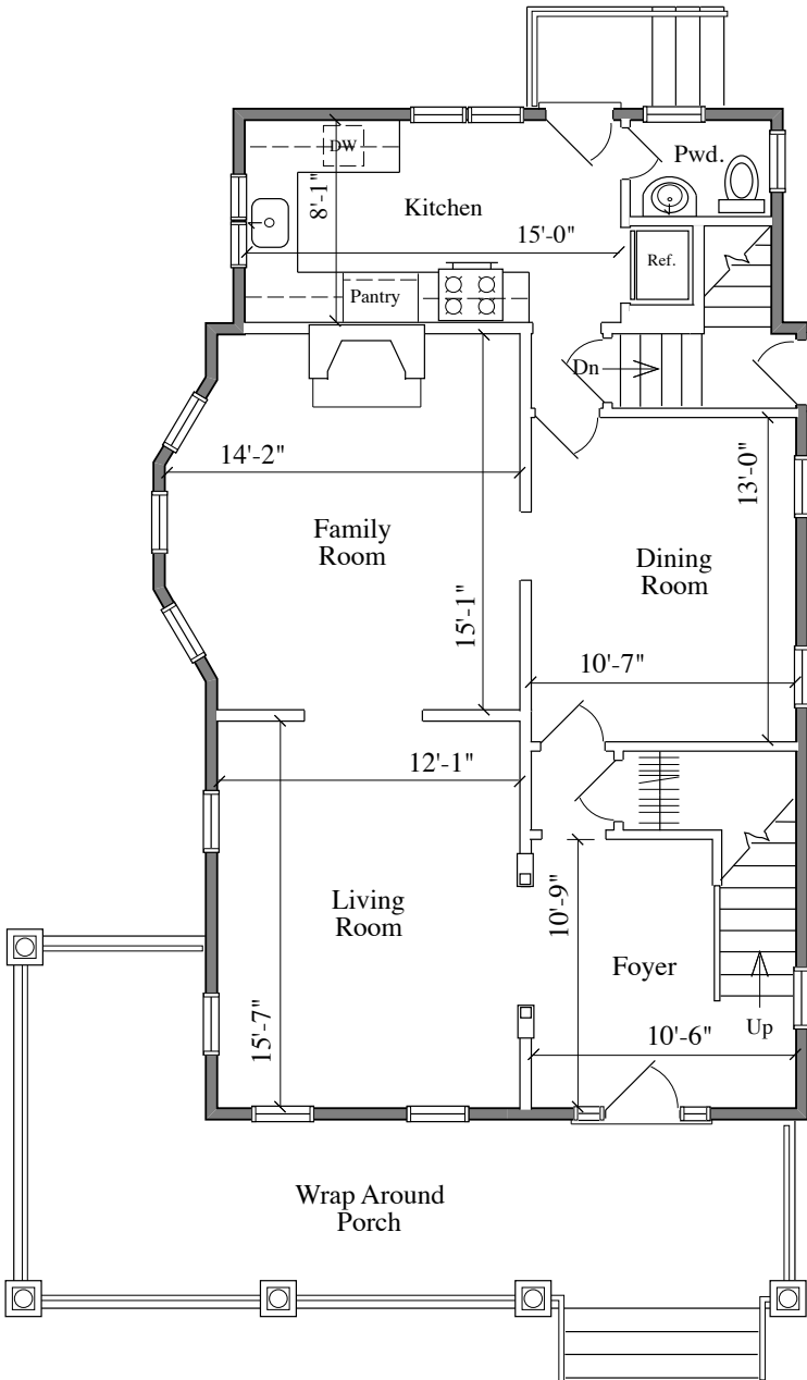
FIRST FLOOR 990 SQ. FT.
