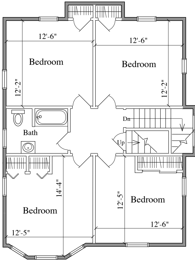
SECOND FLOOR 910 SQ. FT.
