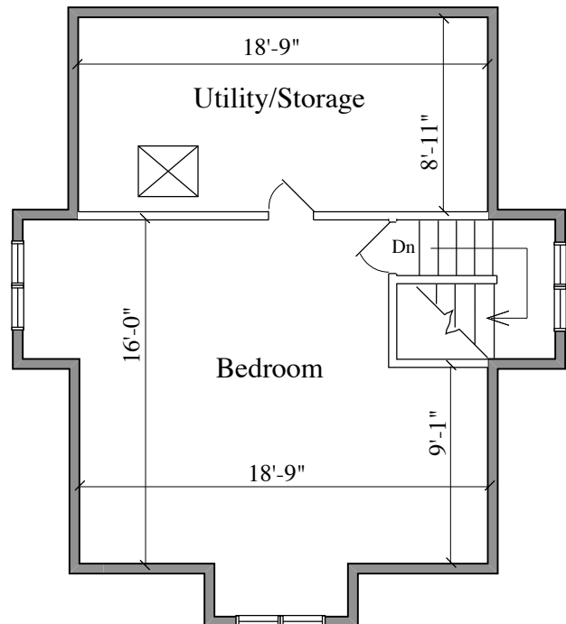
THIRD FLOOR 575 SQ. FT.
