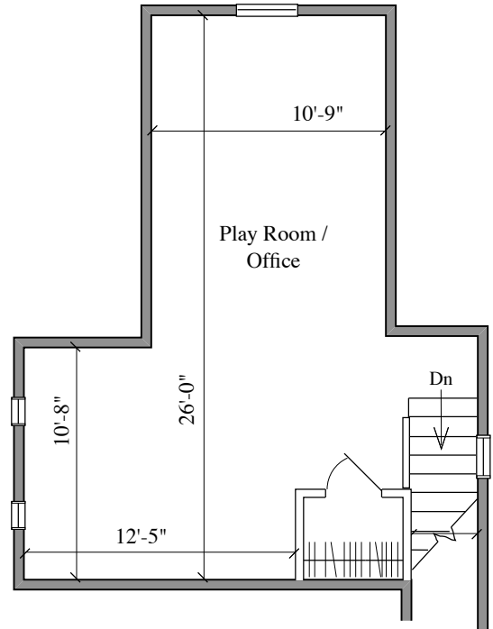
THIRD FLOOR 435 SQ. FT.
