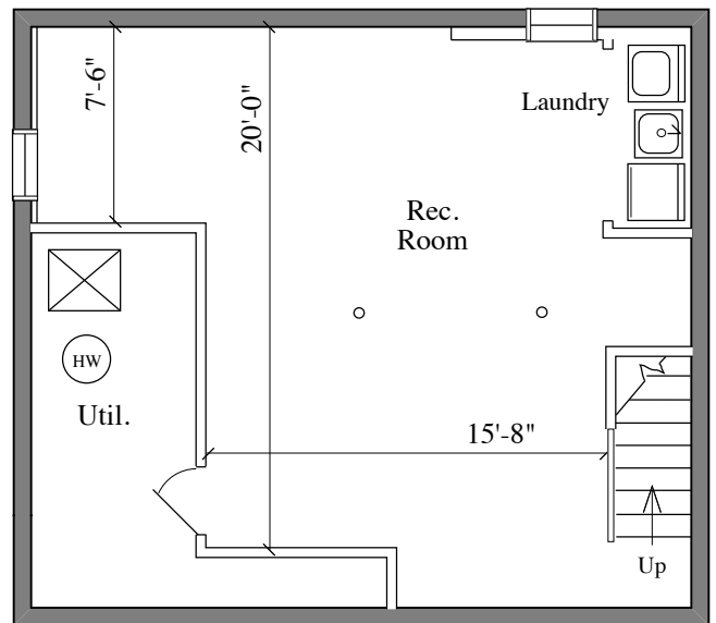
BASEMENT 625 SQ. FT.
