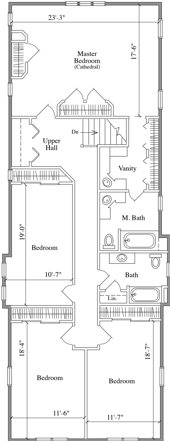
SECOND FLOOR 1,710 SQ. FT.
